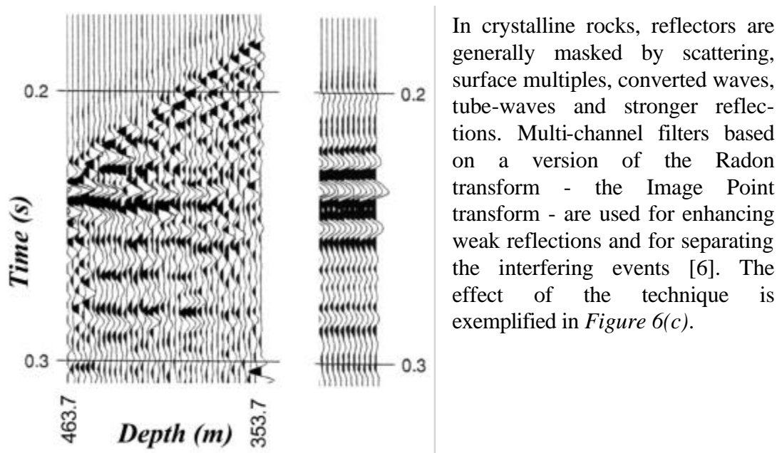
Figure 5. Zero-offset and stacked sections.
